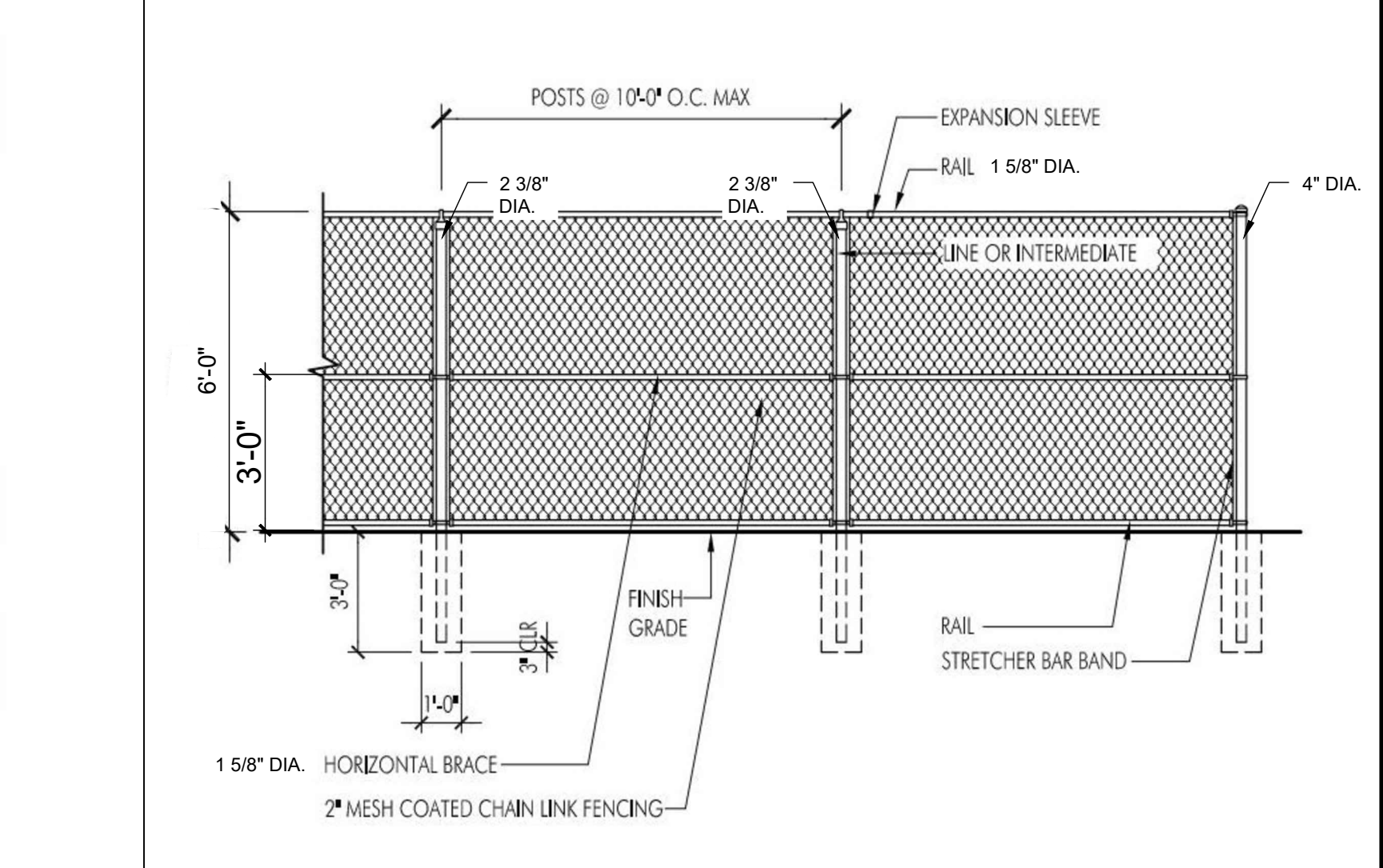
CHAIN LINK FENCE SCALE: 1/2"=1'-0" 2
