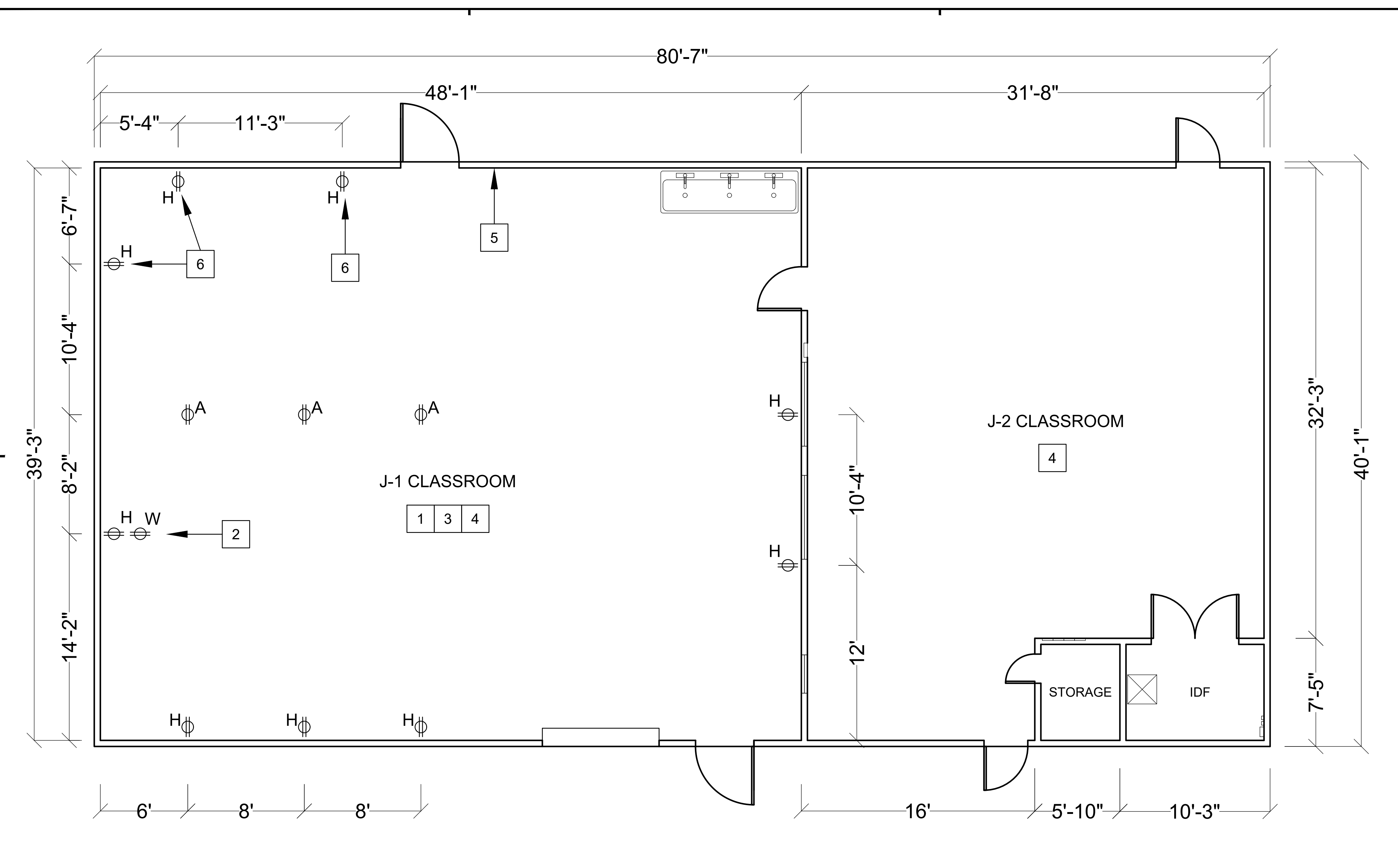
ELECTRICAL PLAN - BUILDING J, CLASSROOM 1 & 2 SCALE: 1/4" = 1'-0" 4
