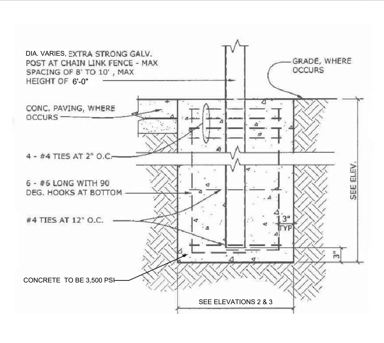
FENCE / GATE POST FOOTING SCALE: 1/2"=1'-0" 8
