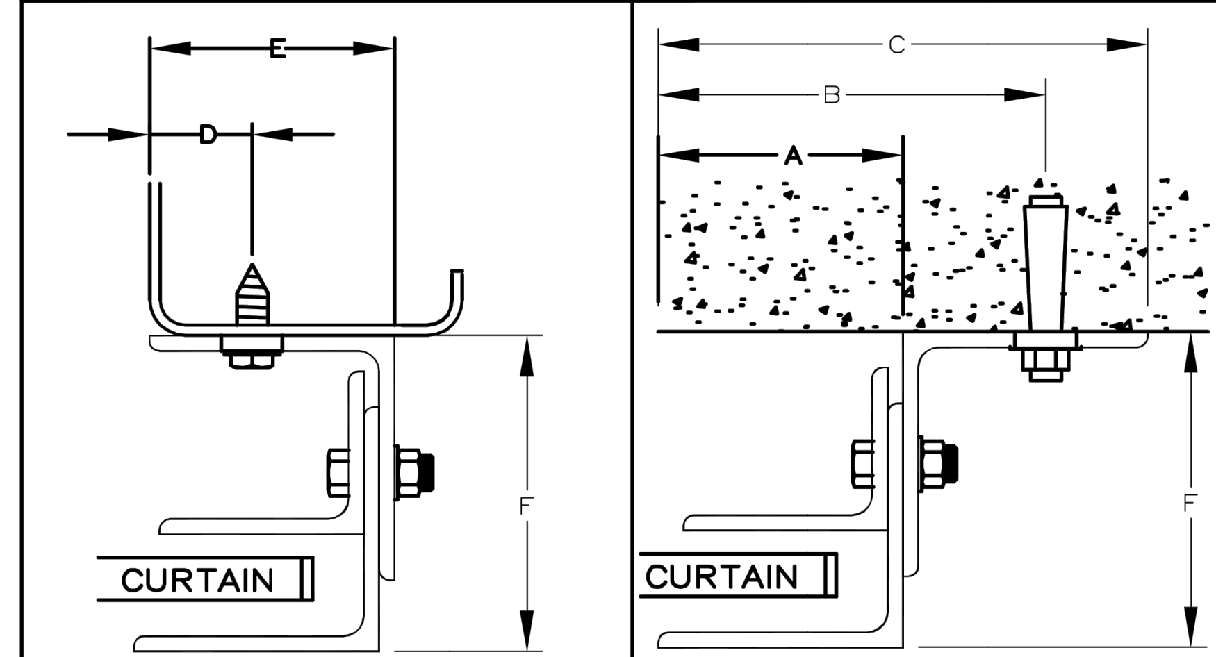
Z-GUIDE FOR CONCRTE MASONRY
