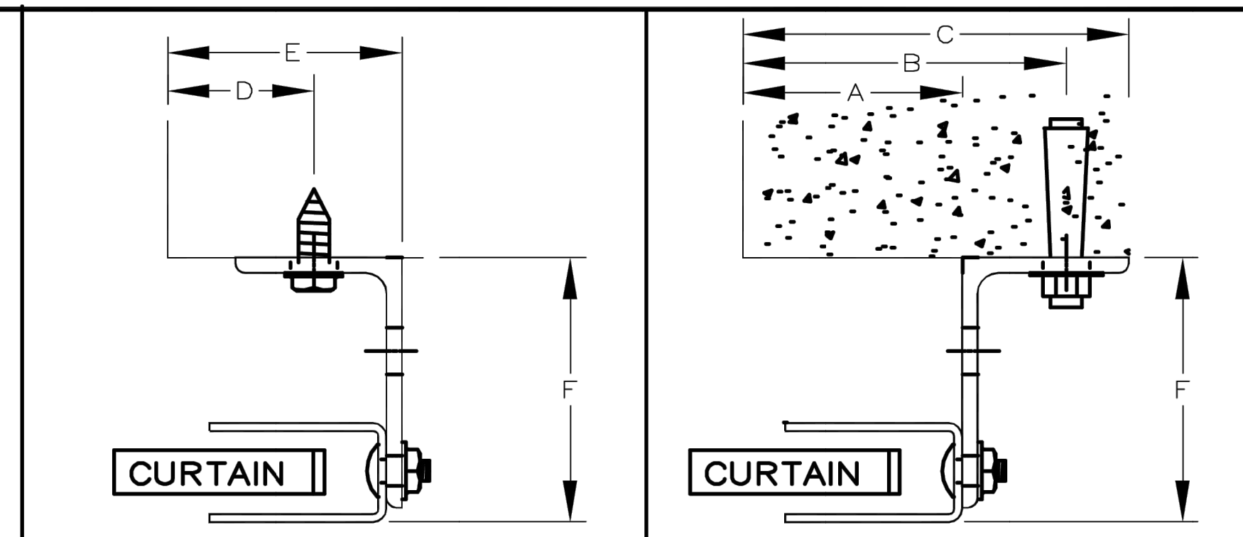
Z-GUIDE FOR CONCRTE MASONRY
