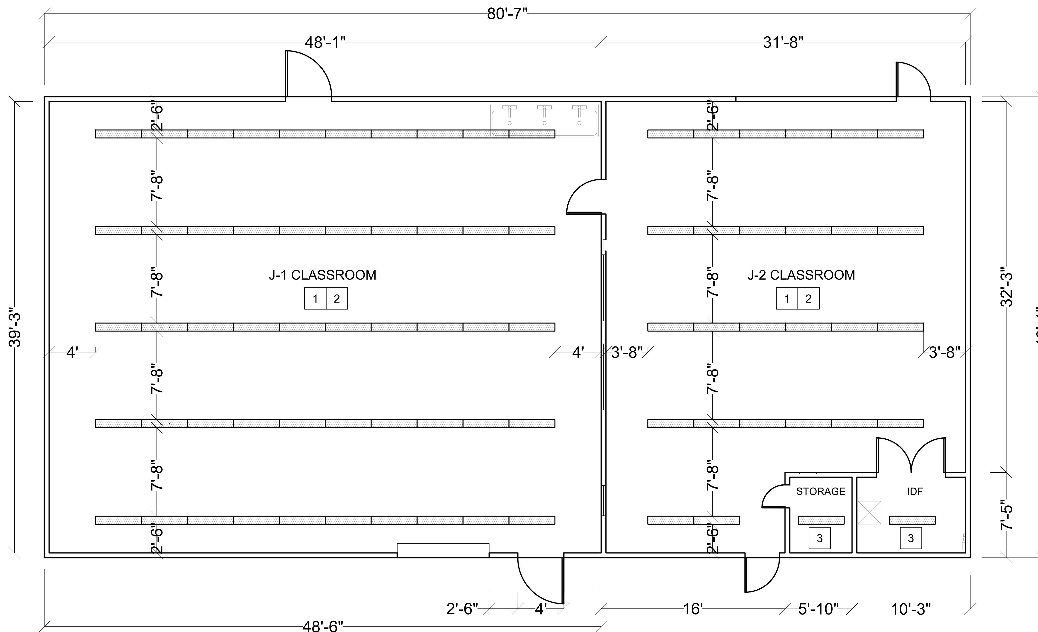
LIGHTING PLAN - BUILDING J, CLASSROOM 1 & 2
