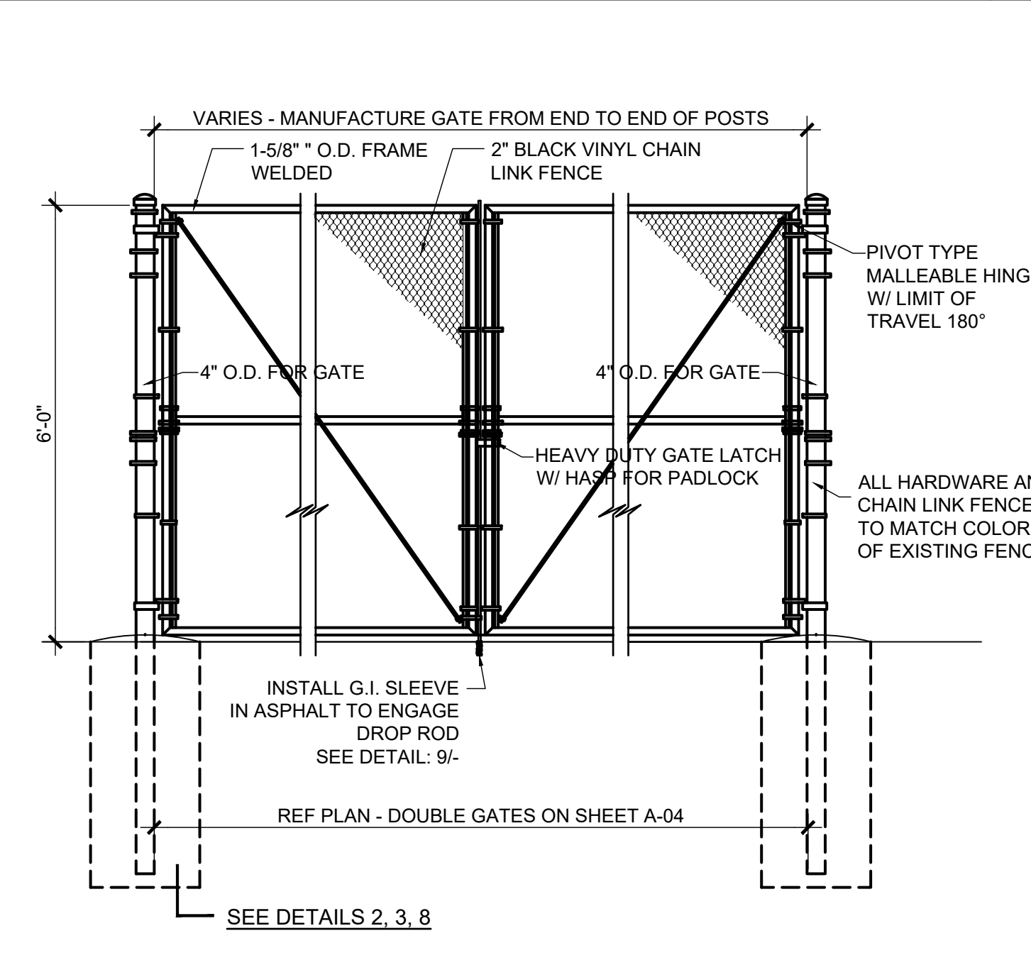
BLACK VINYL FENCE GATES SEE SHEET 07 SCALE: 1/2"=1'-0" 5
