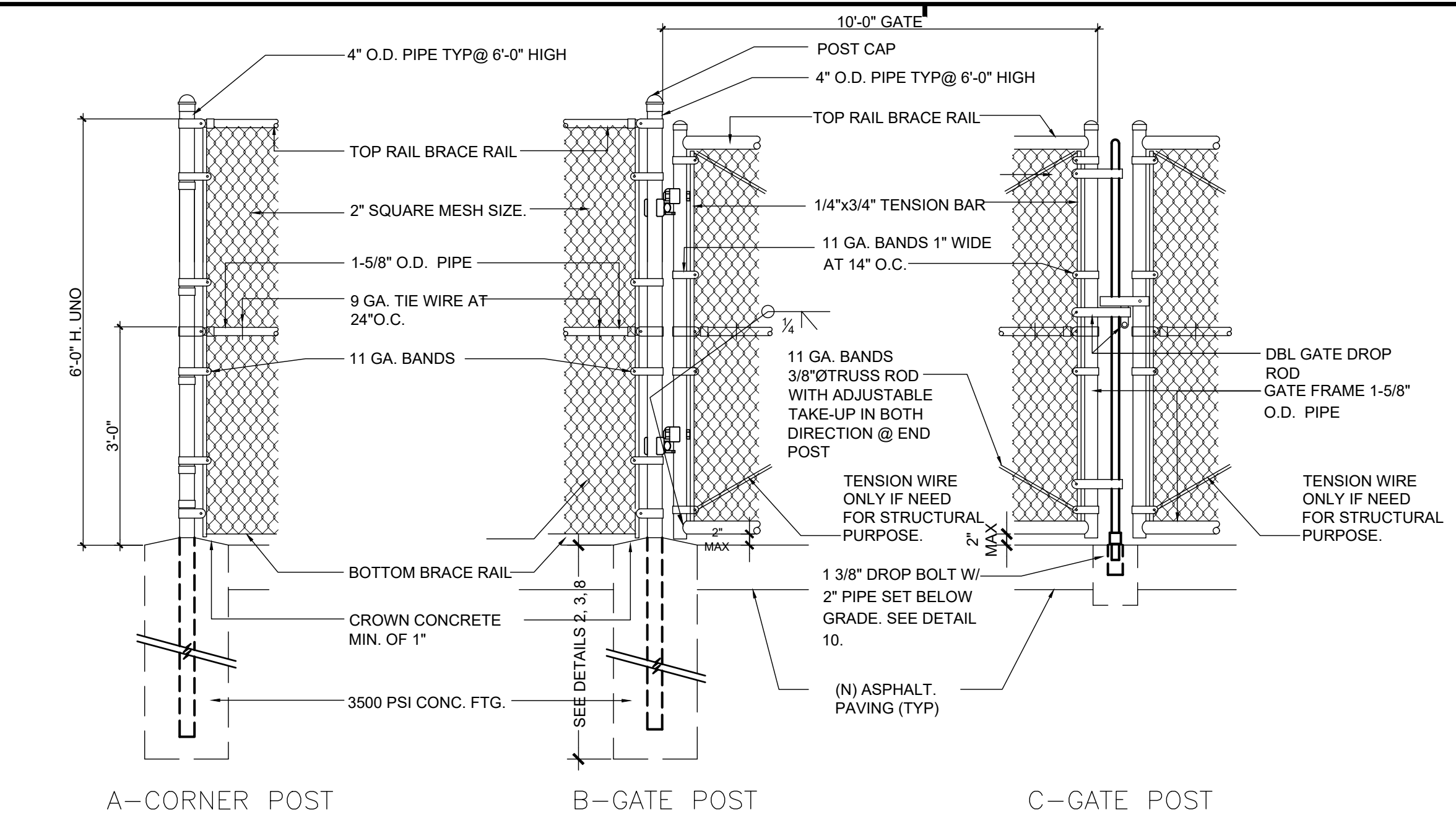
FENCE AND POST DETAILS SCALE: 3/8"=1'-0" 1
