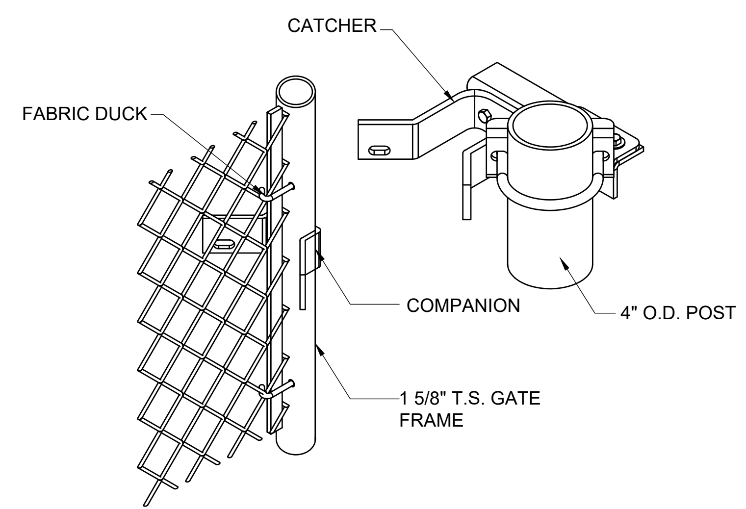
CATCHER ASSEMBLY SCALE: 3/4"=1'-0" 6
