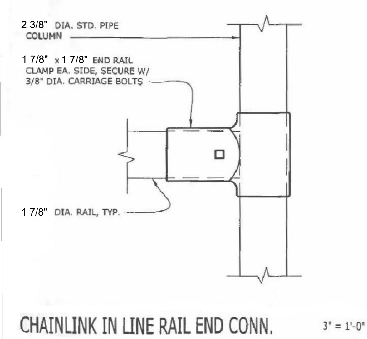
CHAINLINK IN LINE RAIL END CONN. SCALE: 3"=1'-0" 10
