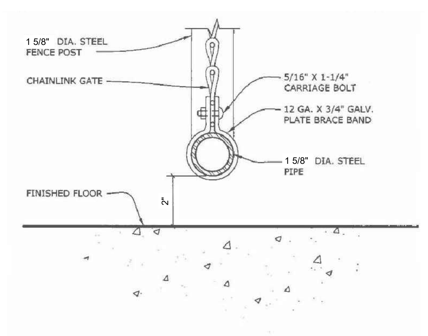
CHAIN LINK GATE THRESHOLD SCALE: 3"=1'-0" 7
