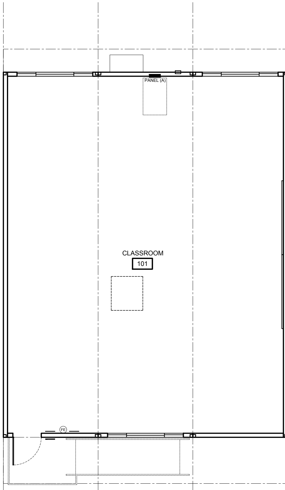
30'x32' CLASSROOM FLOOR PLAN FOR FOURTH USED PORTABLE WITH TBD INSTALLATION DATE (Phase 2)
